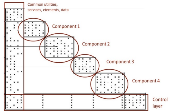
Figure 1: DSM of an ideal code base
